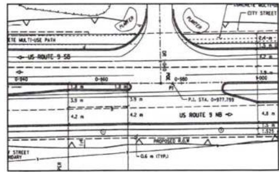
Figure 3.3.4.12: Median with turn bays.
