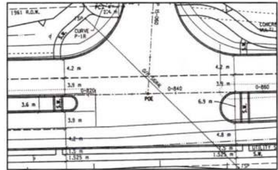
Figure 3.3.4.11: Forced left turn.
