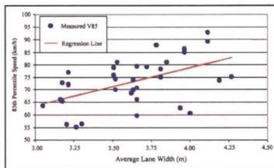
Figure 2.8: Speed in relation to lane width. 20
