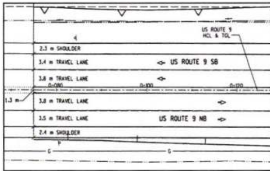
Figure 3.3.4.9: Flush median.
