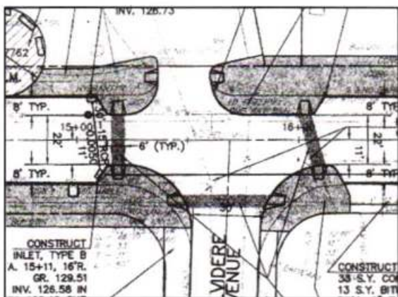
Figure 3.2.2.12: Belvidere Avenue intersection.
