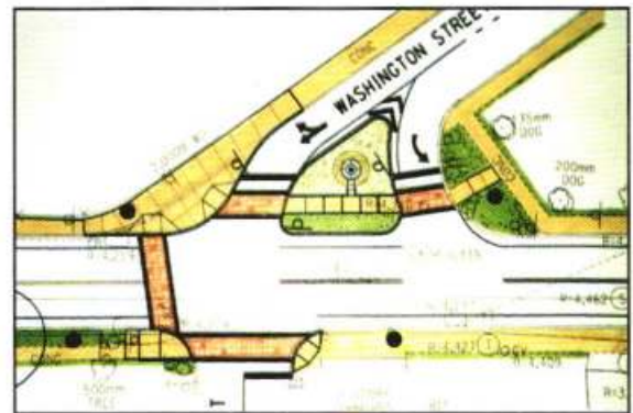
Figure 3.3.3.9: Proposed intersection with Washington and Burke Streets.
