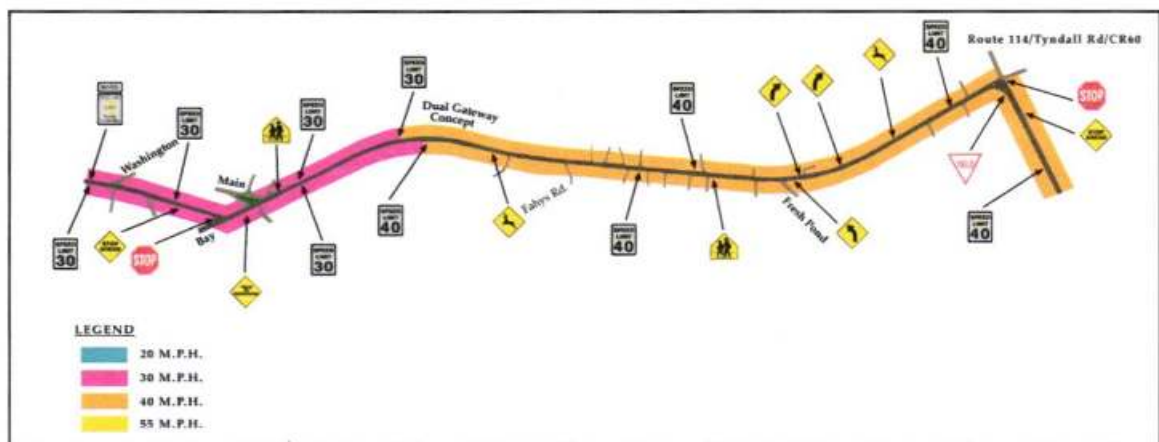
Figure 3.3.3.3: Project plan.
