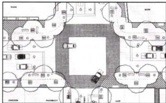
Figure 3.2.1.15: Proposed Prospect Street intersection.
