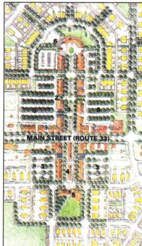
Figure 3.2.4.8: Pedestrian-friendly site plan.
