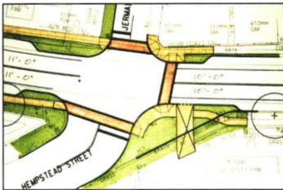
Figure 3.3.3.6: Proposed intersection with Hempstead Street and Jermain Avenue.
