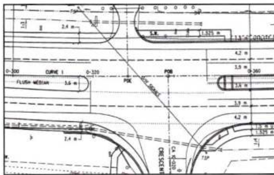
Figure 3.3.4.10: Flush to raised median.
