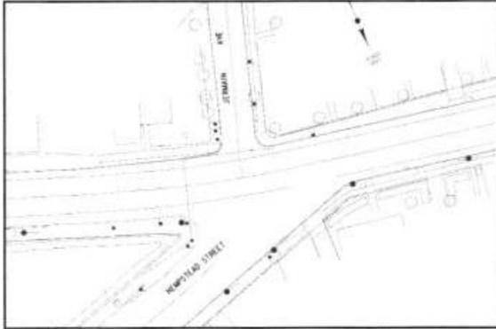
Figure 3.3.3.5: Existing intersection with Hempstead Street and Jermain Avenue.
