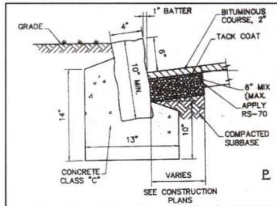
Figure 3.2.2.20: Curb detail.
