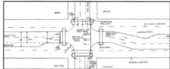
Figure 3.3.6.14: Lane shift plan.
