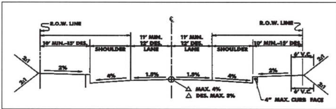
Figure 2.7: Typical section for a two-lane highway from New Jersey's Roadway Design Manual.
