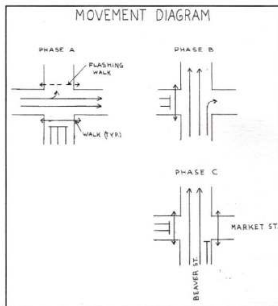
Figure 3.3.6.19: Typical signal timing.
