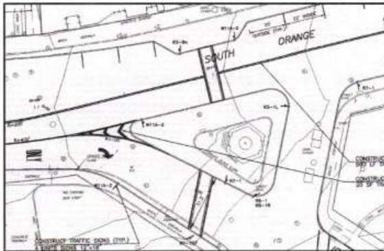
Figure 3.2.3.13 Center island reconstruction at Irvington Avenue/Academy Street.
